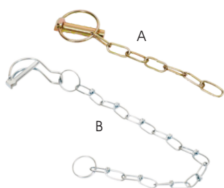
A. Linch Pin With Chain Size : 4.5mm to 12mm B. Tube Linch Pin with Chain Size : 6mm to 12mm
