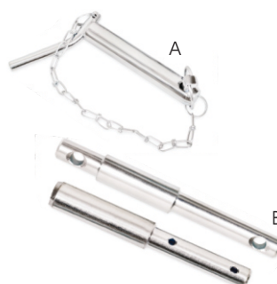
A. Bent Handle Pins with Chain Size : 16mm to 32mm B. Implement Pins Cat 1, 2, 3
