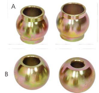
A. Top Link Balls B. Lower Link Balls Cat 1, 2, 3
